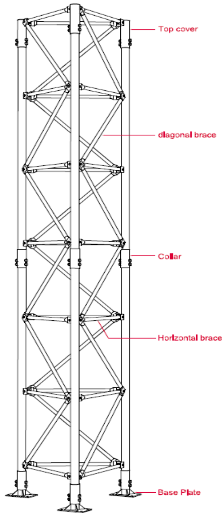
Assembled mast
