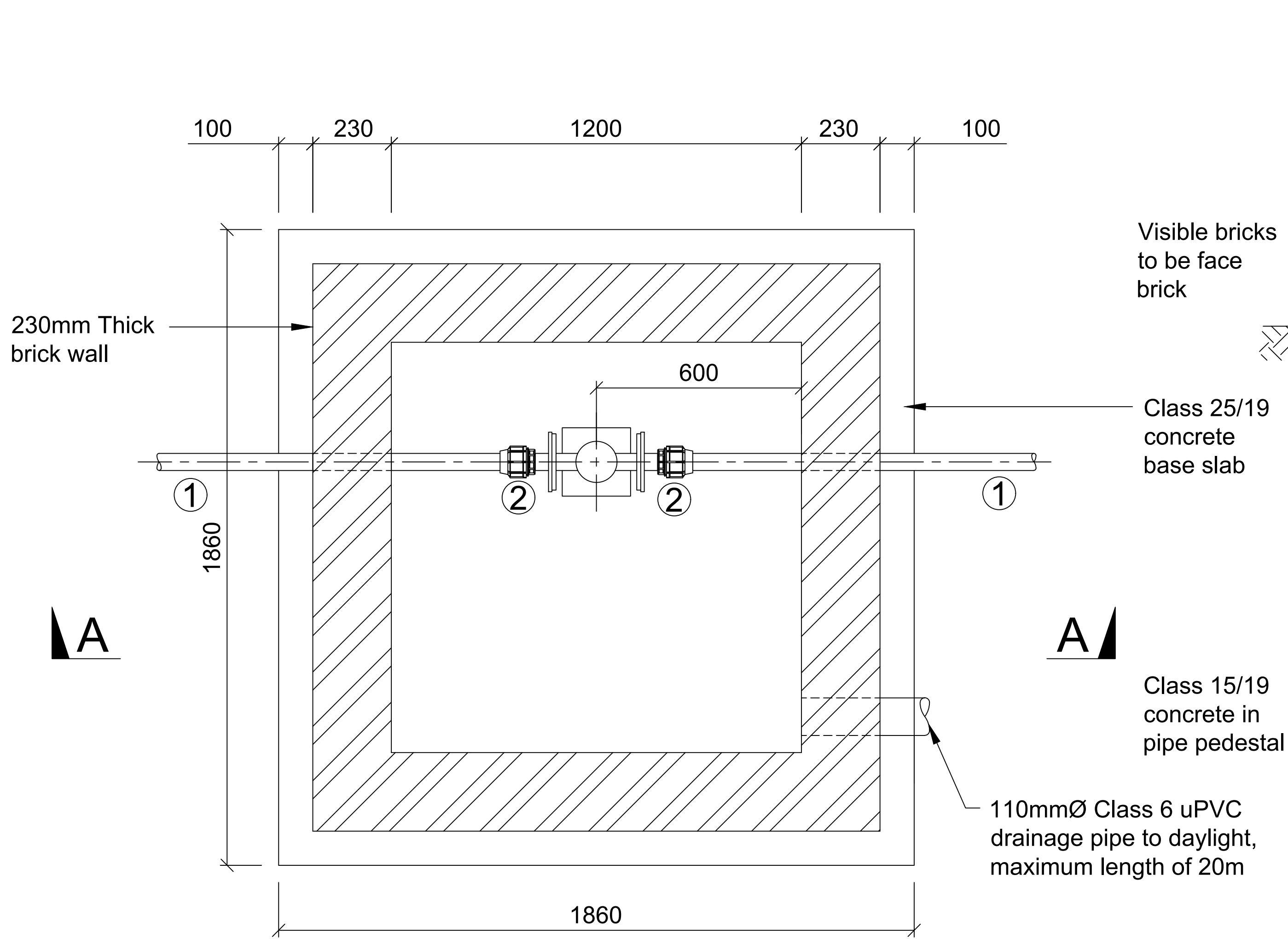
FLOOR PLAN 1:20
